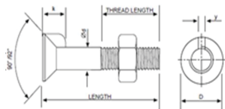
COUNTERSUNK NIB BOLT
