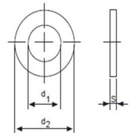
FLAT WASHER
