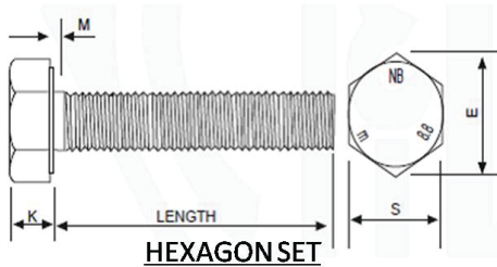
HEXAGON SET
