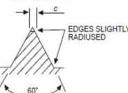
THREAD PROFILE
