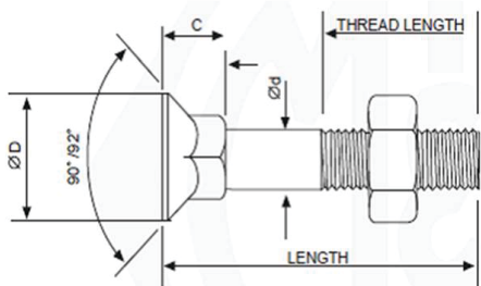
COUNTERSUNK SQUARE BOLT
