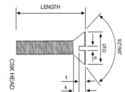
CSK HEAD
