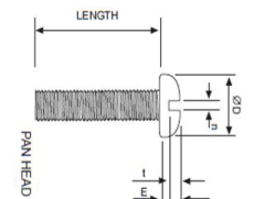
PAN HEAD
