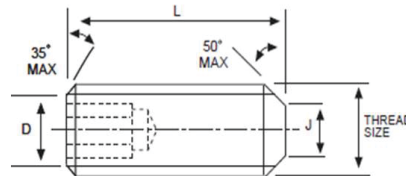
GRUB SCREW
